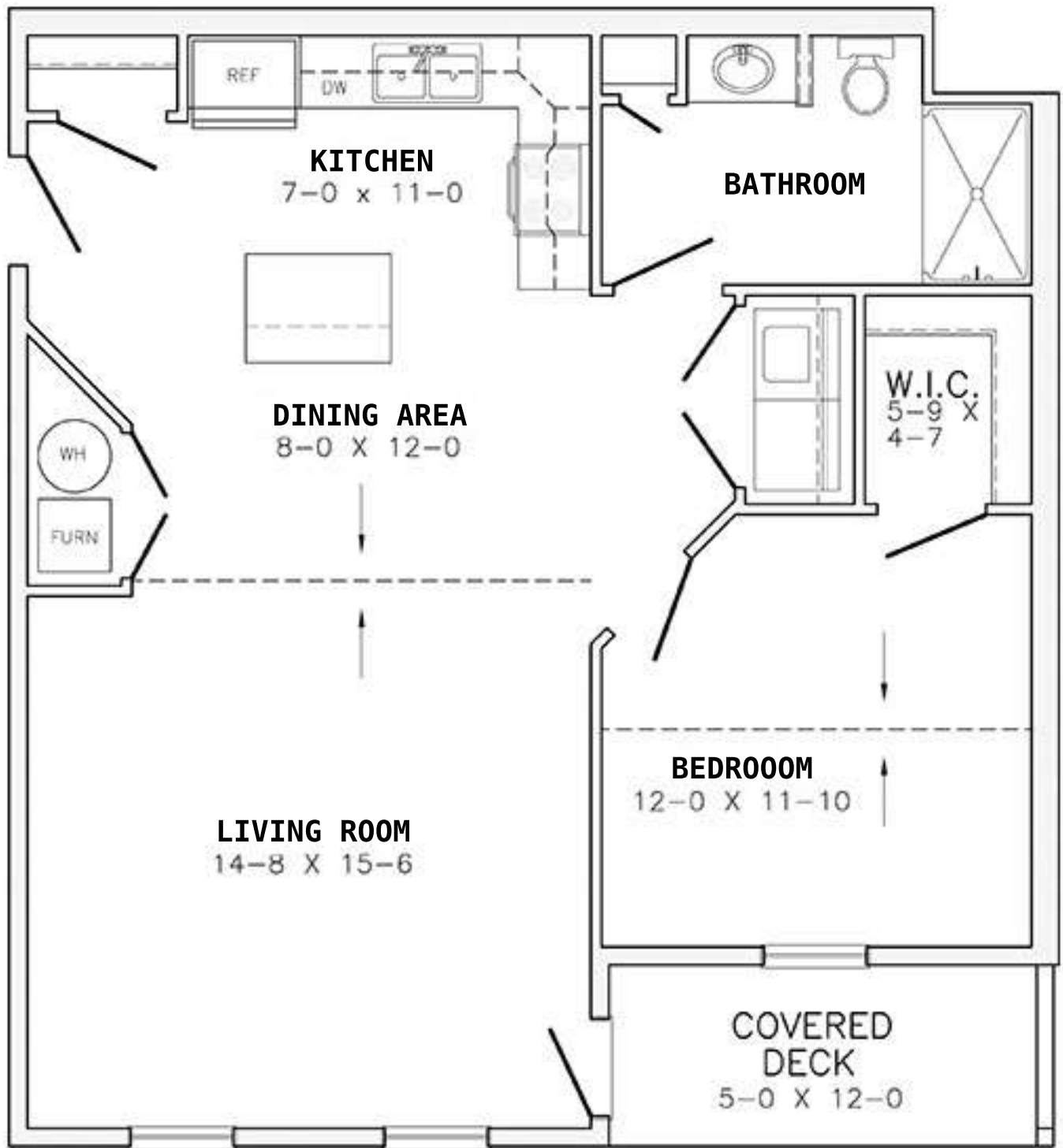
VAULTED CEILING 1 BEDRM./ 1 BATH FLOOR PLAN 816 S.F.
